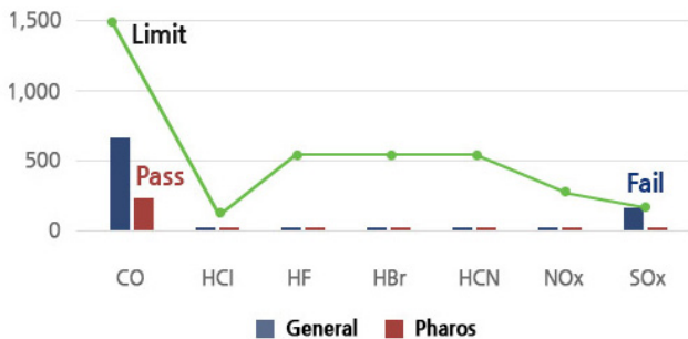
Max. Gas Smoke Density Passed with 49.8 Dm of gas smoke density
