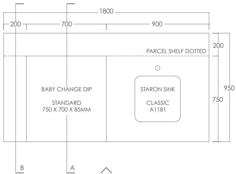
PLAN SCALE 1:20 A3
