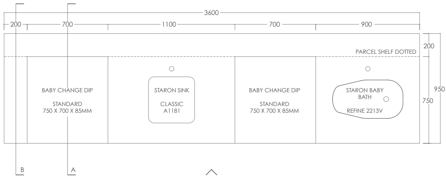
PLAN SCALE 1:20 A3
