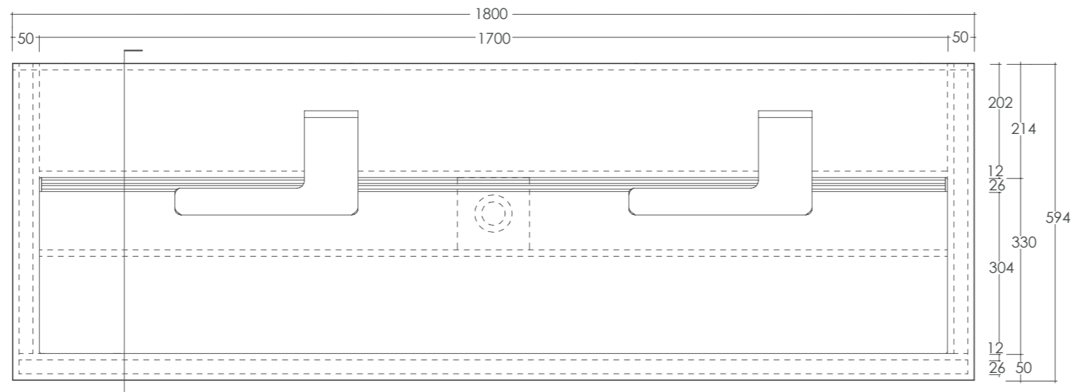
PLAN 2P SCALE 1:10 A3
