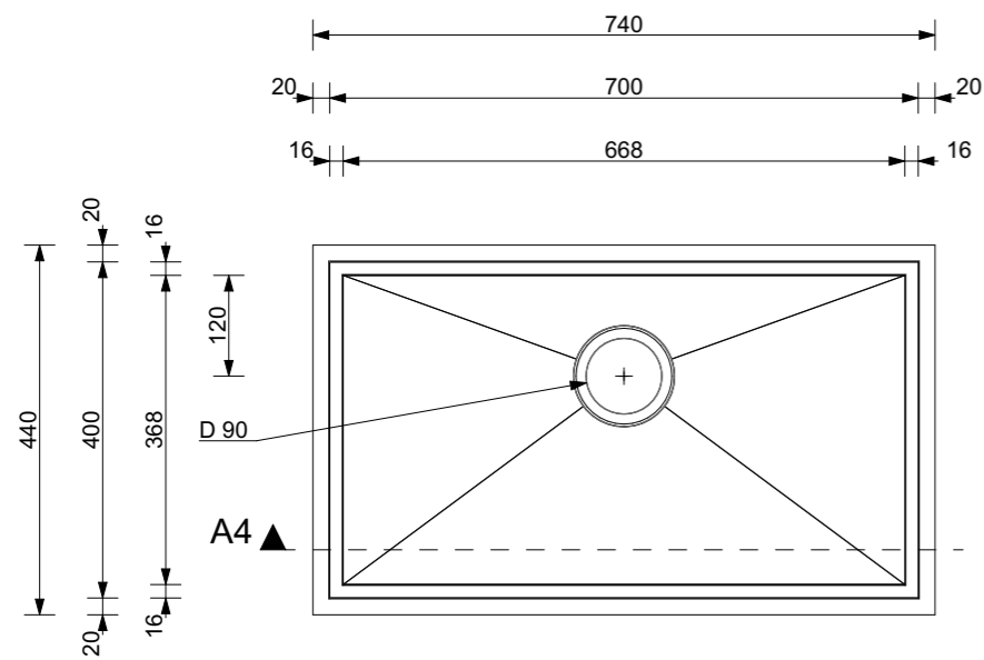
PLAN VIEW
