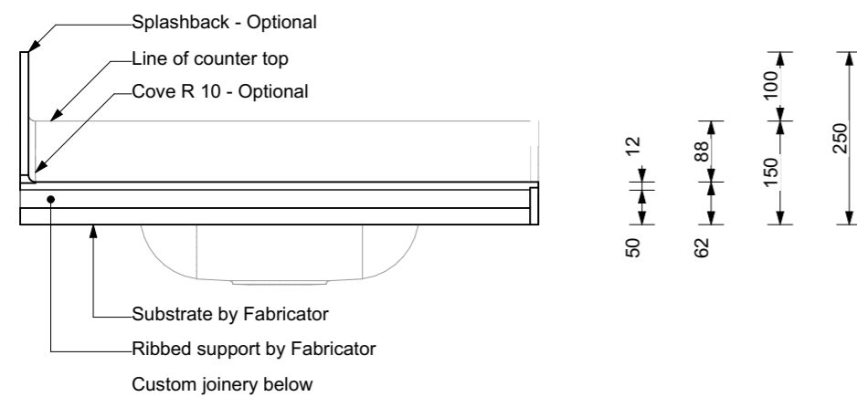
SECTION B-B 1:10
