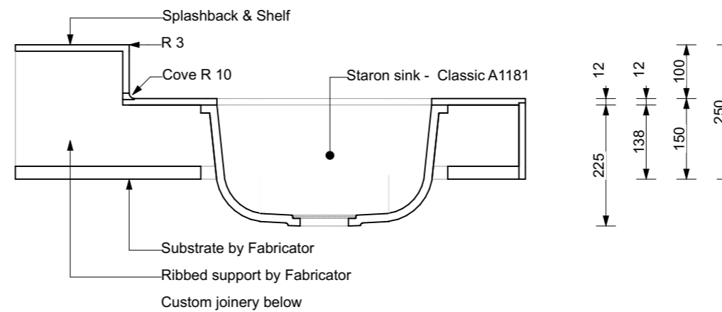
SECTION C-C 1:10
