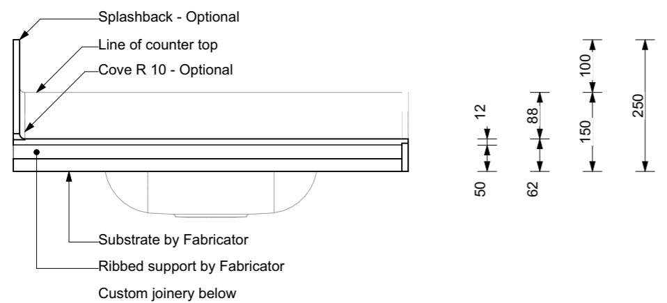
SECTION B-B 1:10
