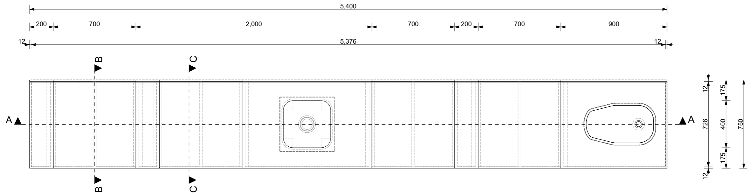
PLAN SCALE 1:20
