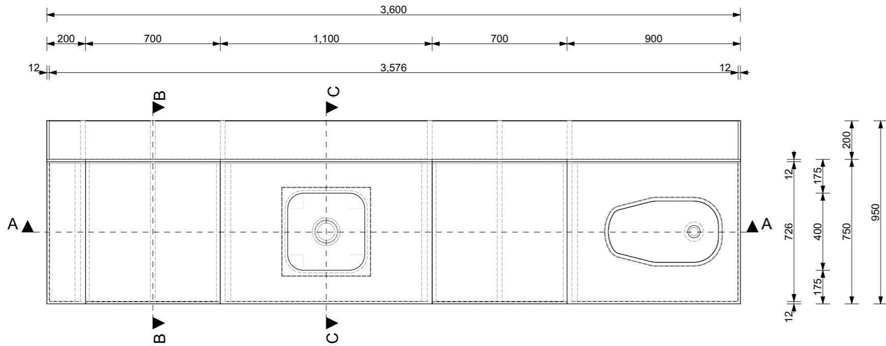
PLAN SCALE 1:20
