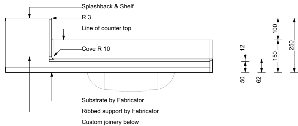
SECTION B-B 1:10
