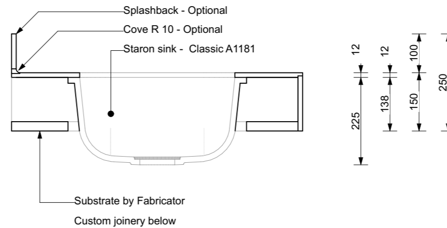
SECTION C-C 1:10
