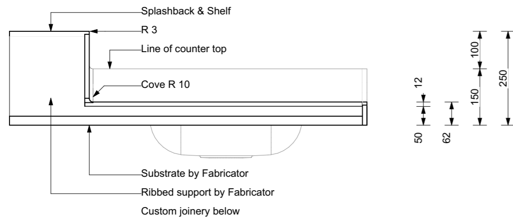
SECTION B-B 1:10
