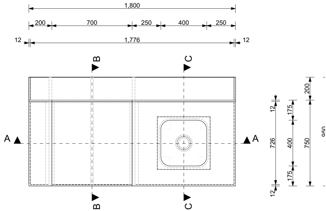
PLAN SCALE 1:20
