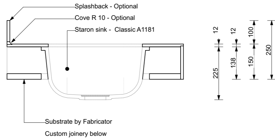
SECTION C-C 1:10
