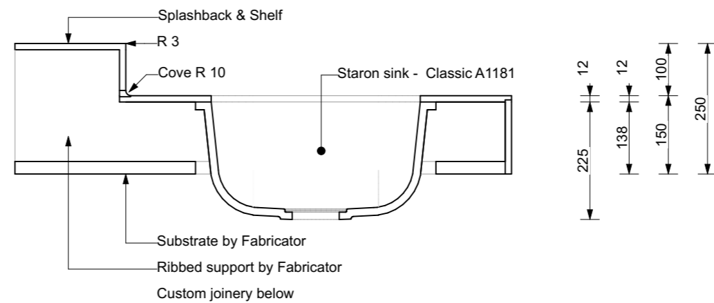
SECTION C-C 1:10
