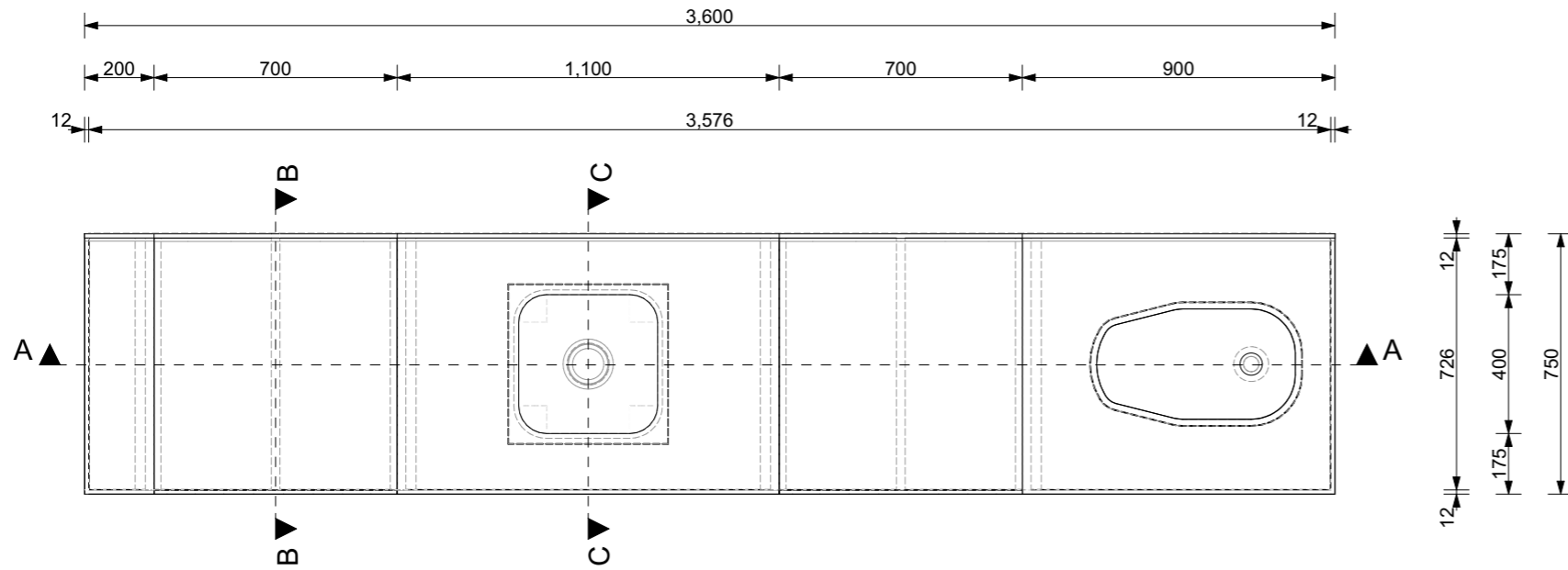
PLAN SCALE 1:20
