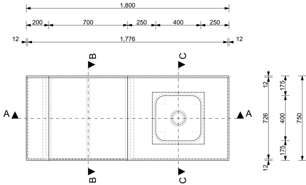
PLAN SCALE 1:20
